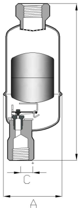
No.11LD DIMENSIONS (MM). MOP(KG/CM 2 ). WT(KG)
