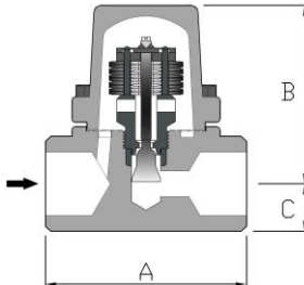
No. SB81 DIMENSIONS (MM). MOP(KG/CM 2 ). WT(KG) (KG)
