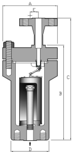
No.1540/1540F DIMENSIONS (MM). MOP (KG/CM 2 ) WT (KG)
